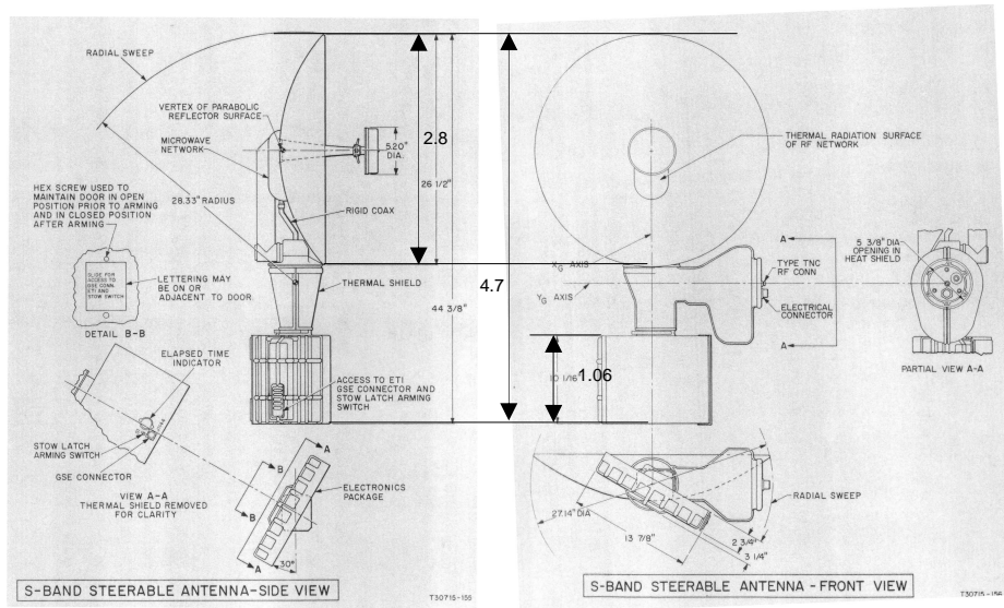
S-Band antenna
