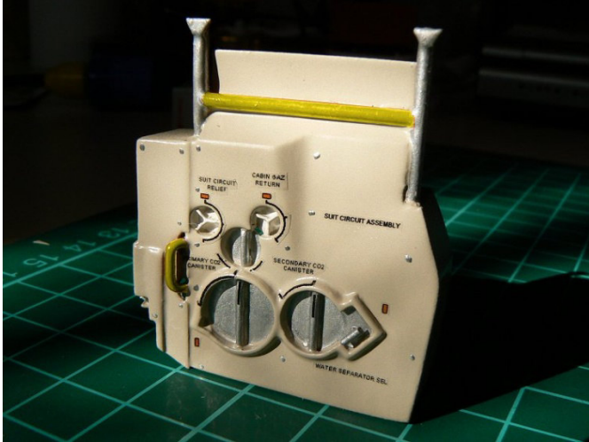
Decals on the Environmental Control System
